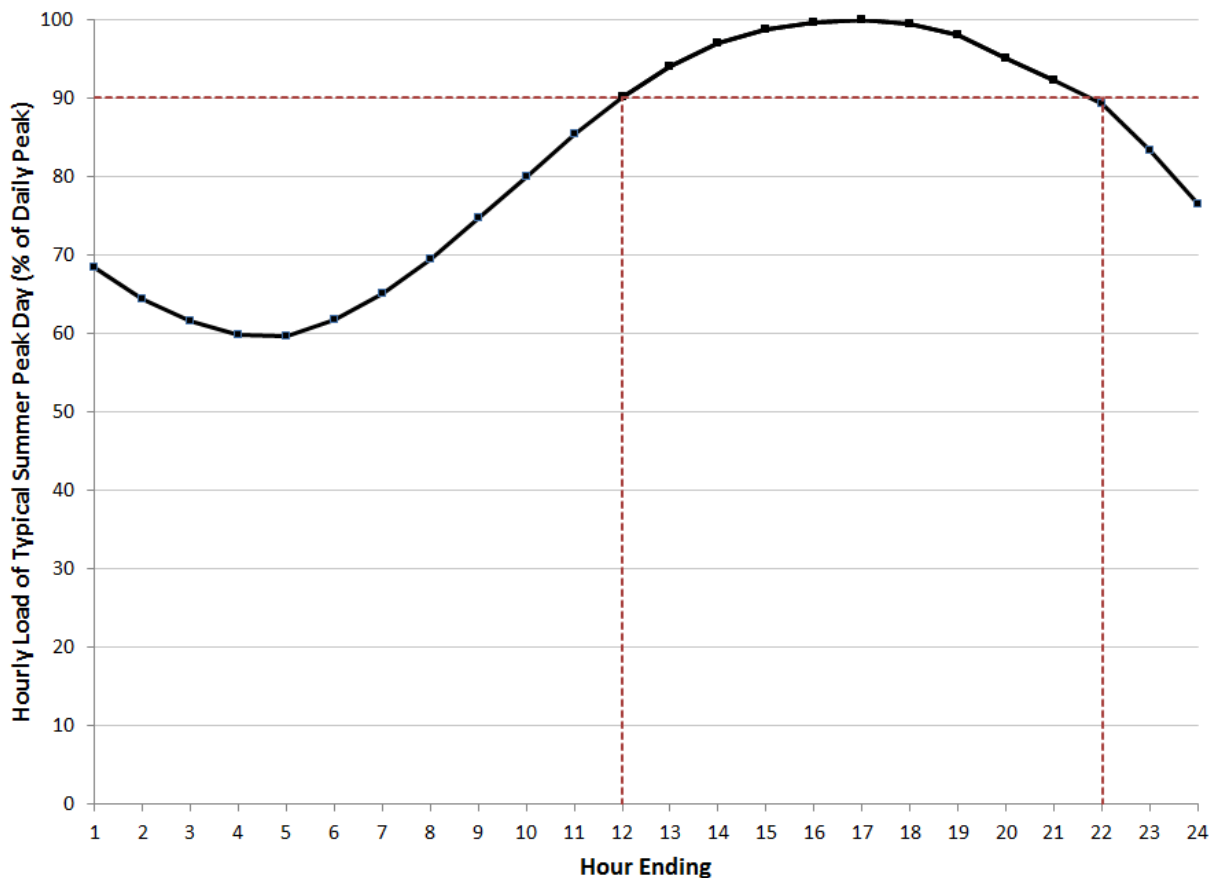
Figure 1 –Summer Weekday Load Shape
