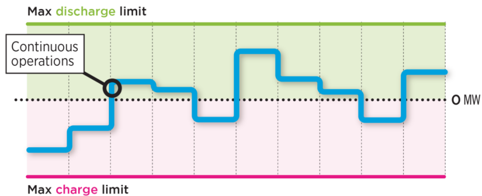
Figure 1: Continuous Mode
