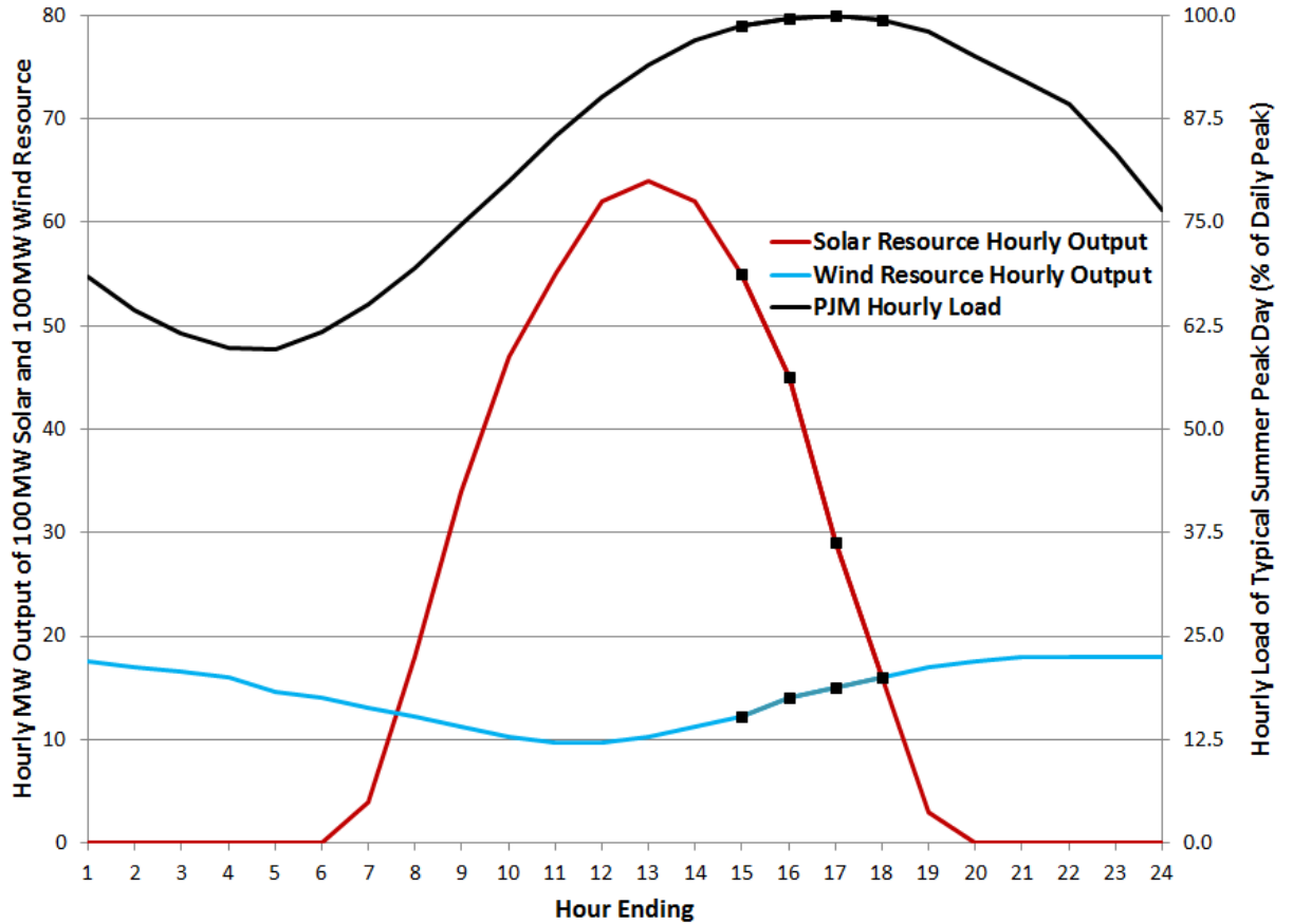
Figure 2 – Average Hourly Output of 100 MW Solar Resource and 100 MW Wind Resource in Summer Period Relative to Summer Weekday Load Shape
