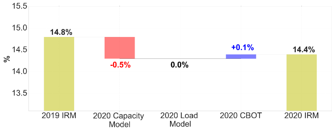
Figure I-2: 2020 Installed Reserve Margin Waterfall Chart
