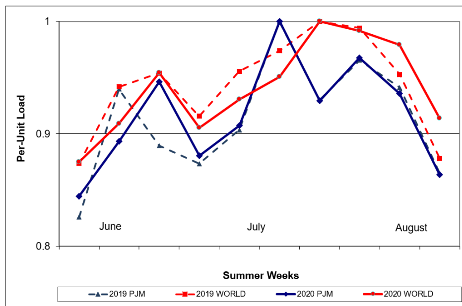
Figure II-3: Expected Weekly Maximum Comparison – 2019 RRS vs. 2020 RRS
