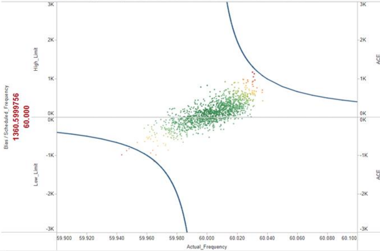
Balancing Authority ACE Limits Performance - 2022-01-16 00:01:00 to 2022-01-17
