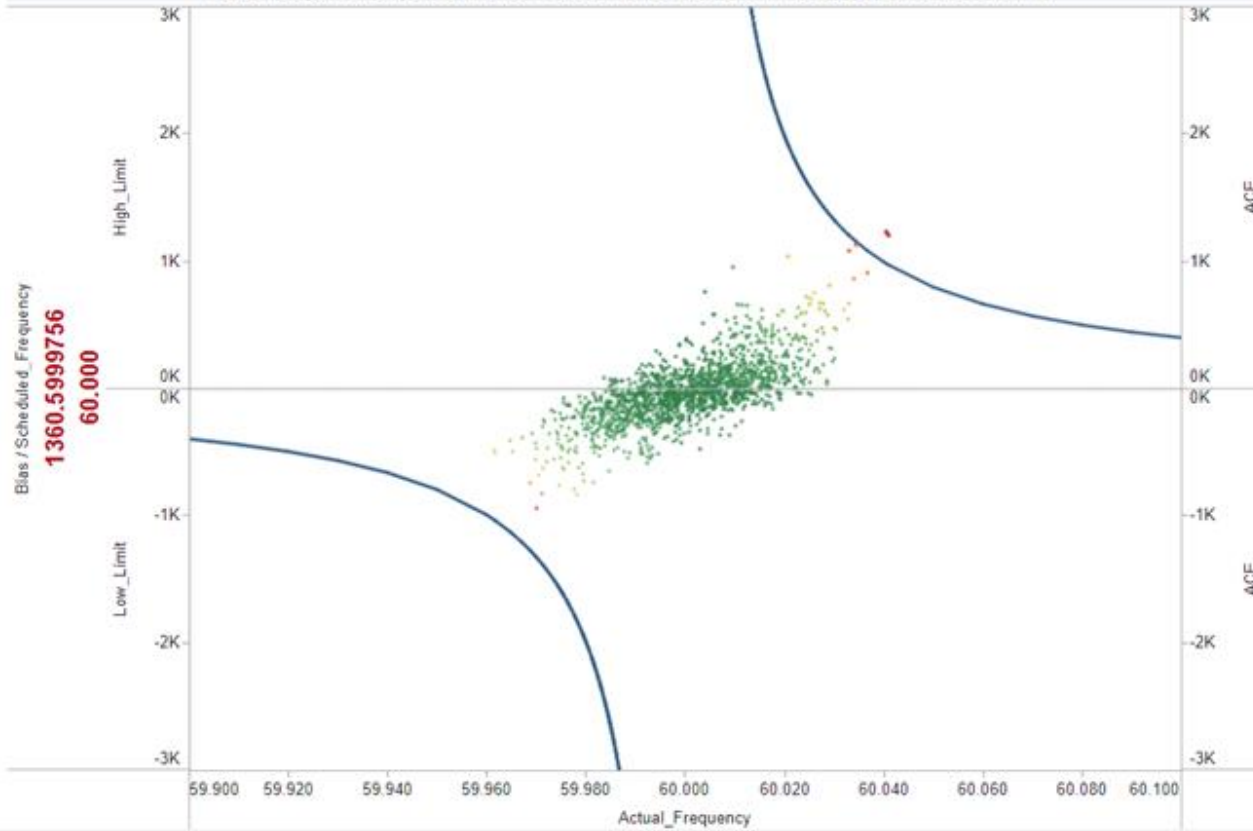
Balancing Authority ACE Limits Performance - 2022-01-15 00:01:00 to 2022-01-16
