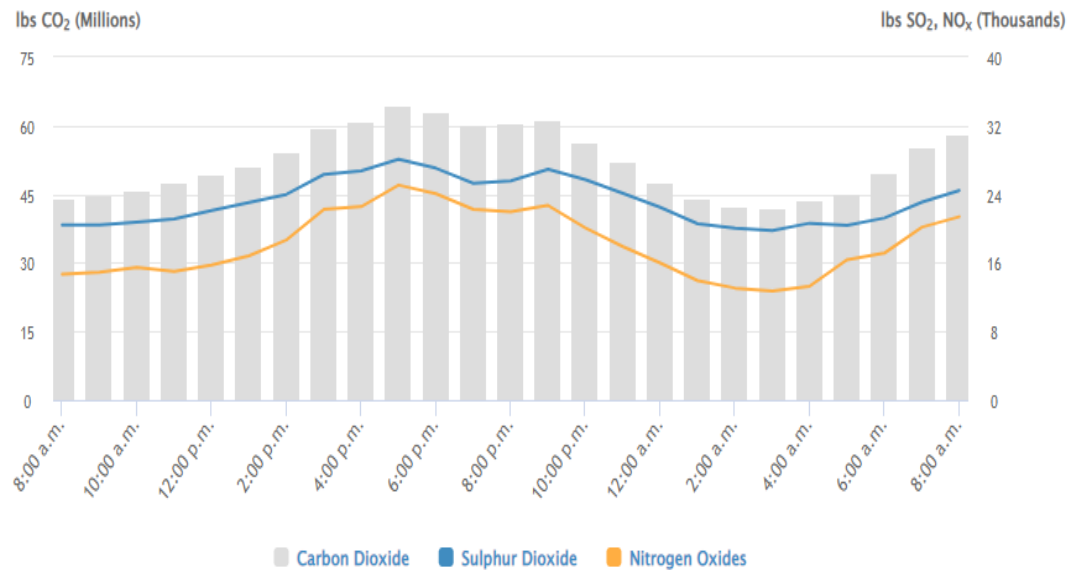
Hourly Emissions for PJM-RTO
