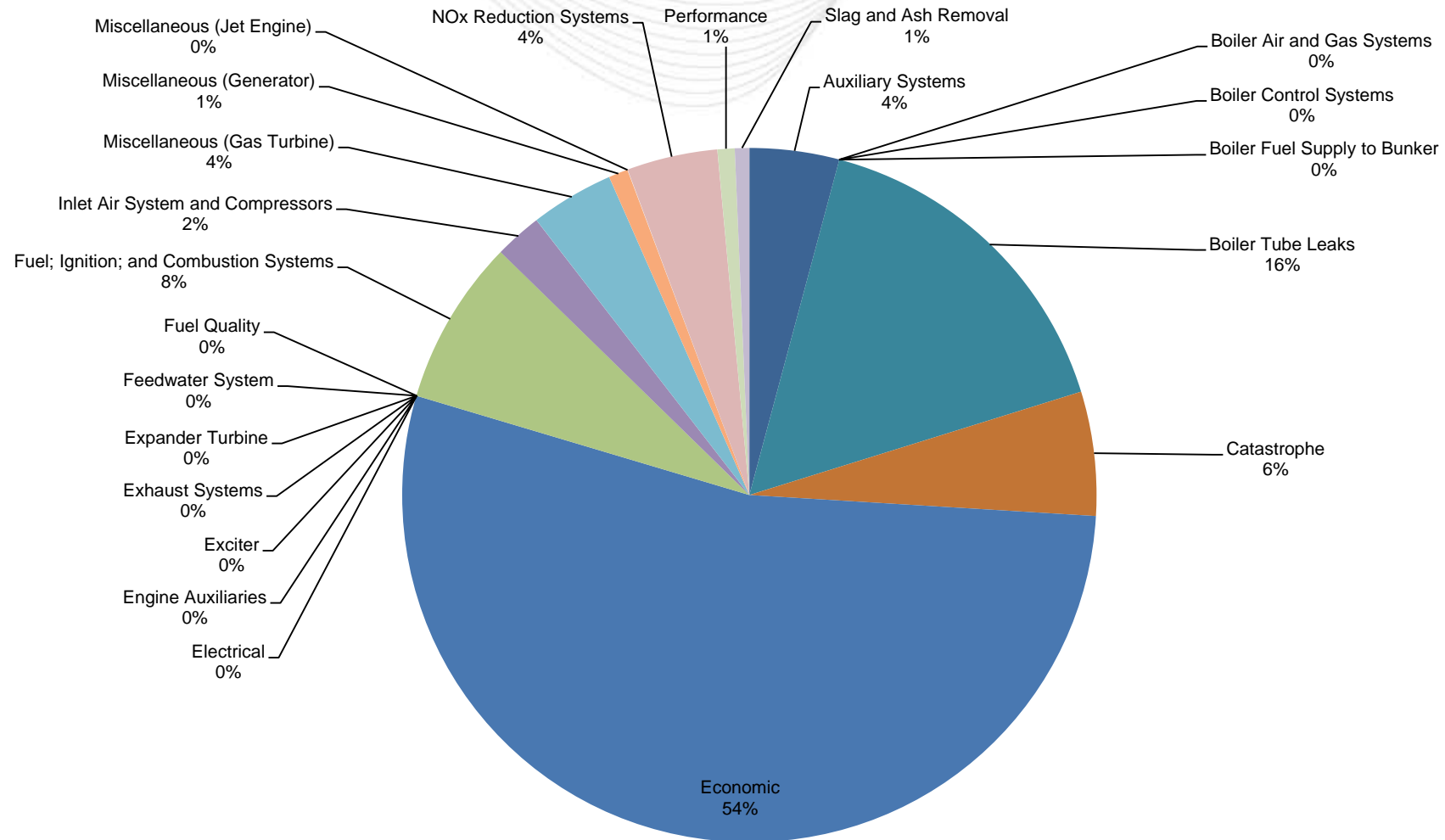
Dual Fuel Capable Start Failure and Forced Outage Causes on 1/28/2014 1800 to 1900
