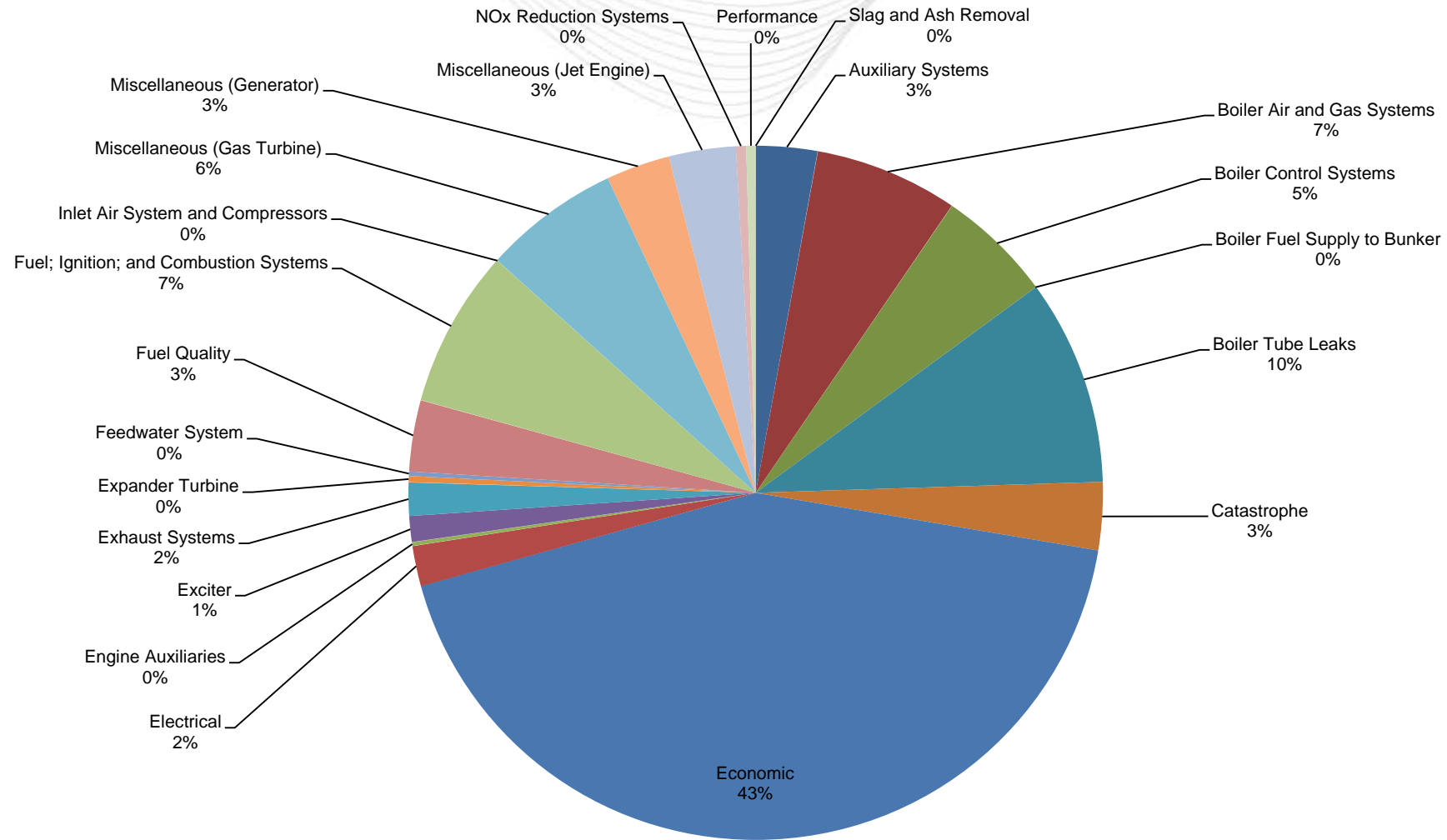
Dual Fuel Capable Start Failure and Forced Outage Causes on 1/7/2014 1800 to 1900
