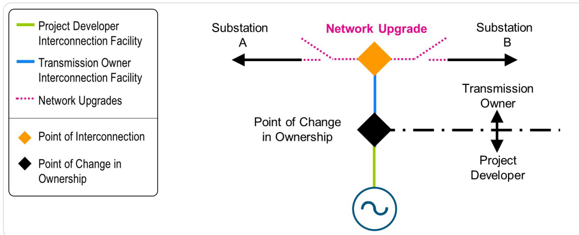
Exhibit XX: Generator Interconnection as a Tap off of an existing Line
