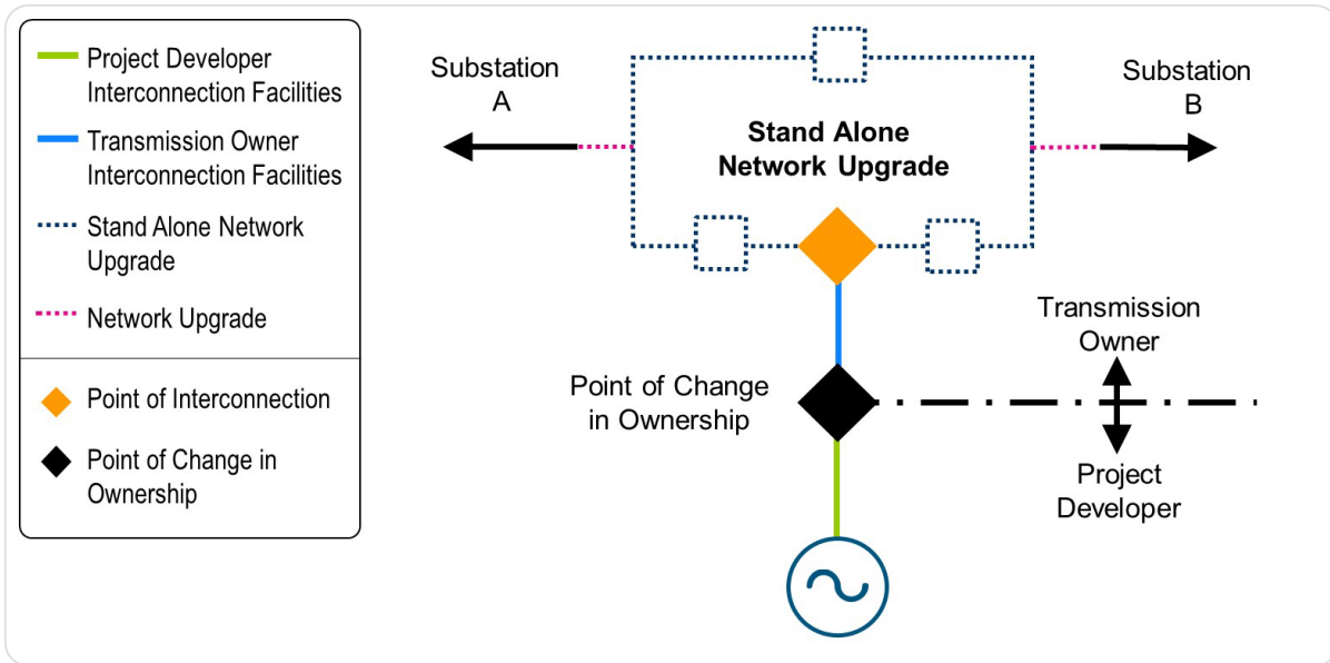
Exhibit XX: Generator Interconnection via new Interconnection Switchyard
