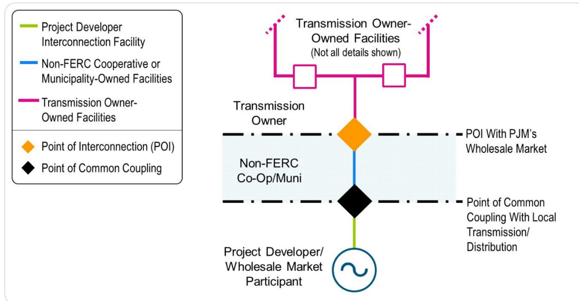
Exhibit XX: Generator Interconnection to a non-FERC Facility
