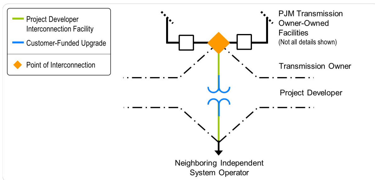
Exhibit XX: Merchant Transmission Interconnection
