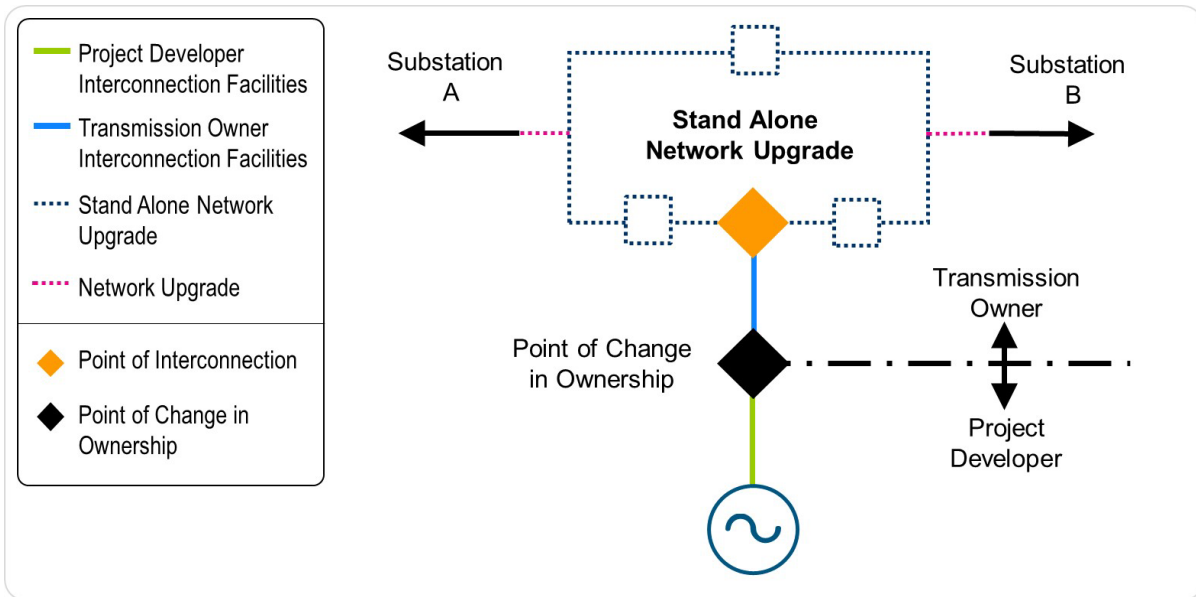
Exhibit XX: Generator Interconnection into Existing TO Substation
