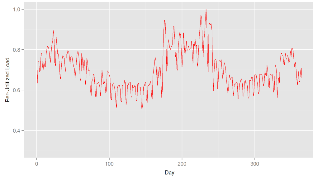
PJM Loads - 2003
