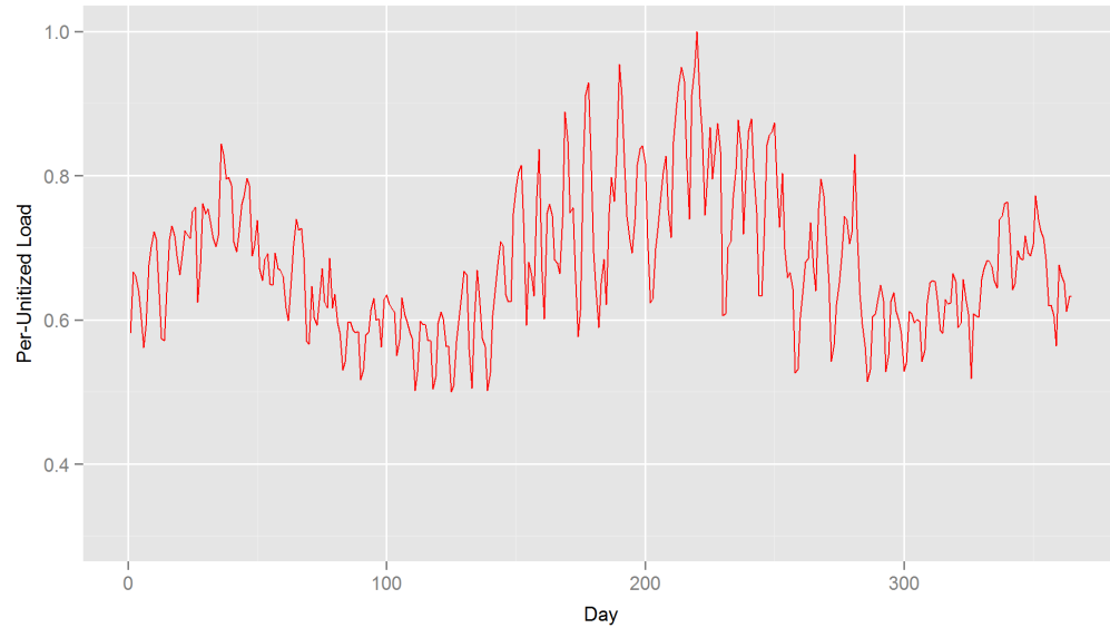
PJM Loads - 2007
