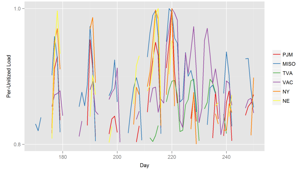
PJM and Neighboring Regions Loads - 2007
