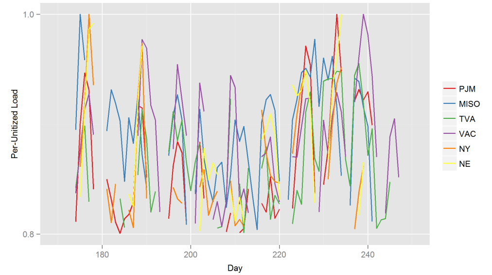
PJM and Neighboring Regions Loads - 2003
