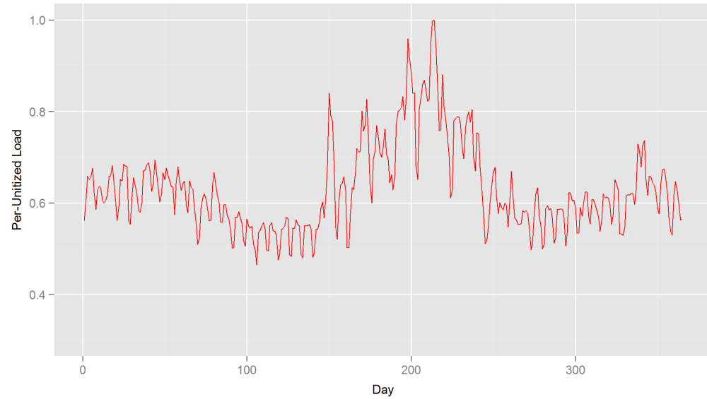
PJM Loads - 2006
