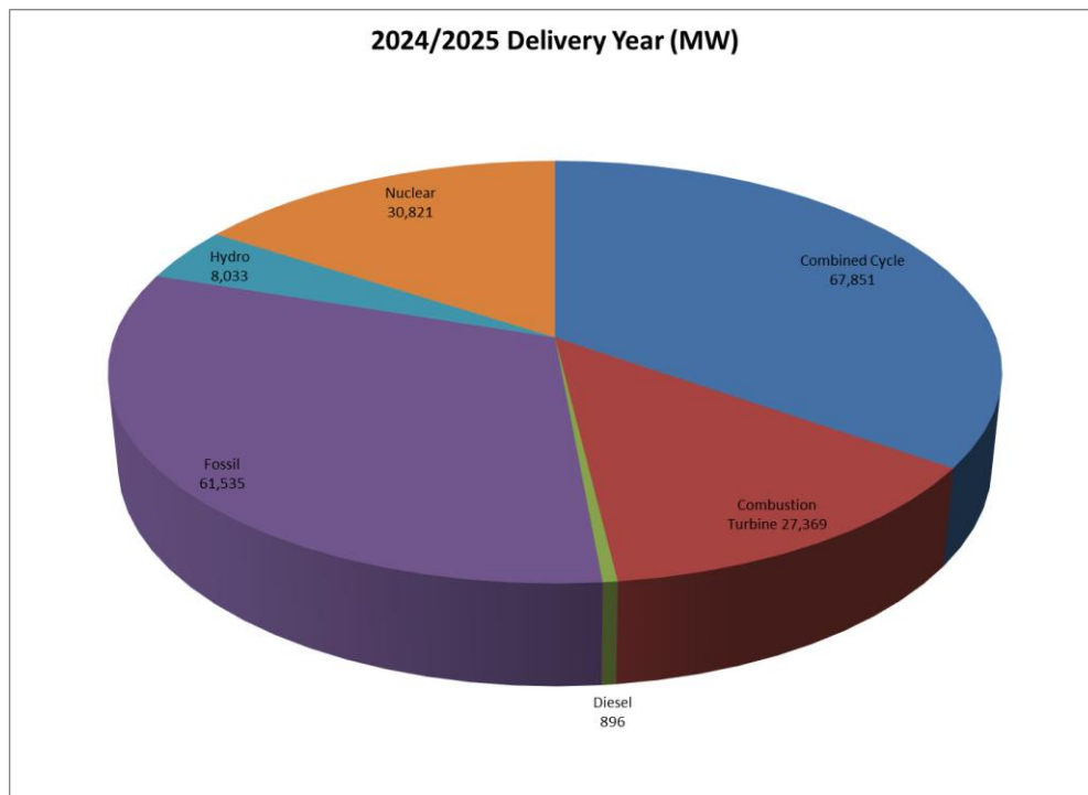
Figure II-1: PJM RTO Capacity
