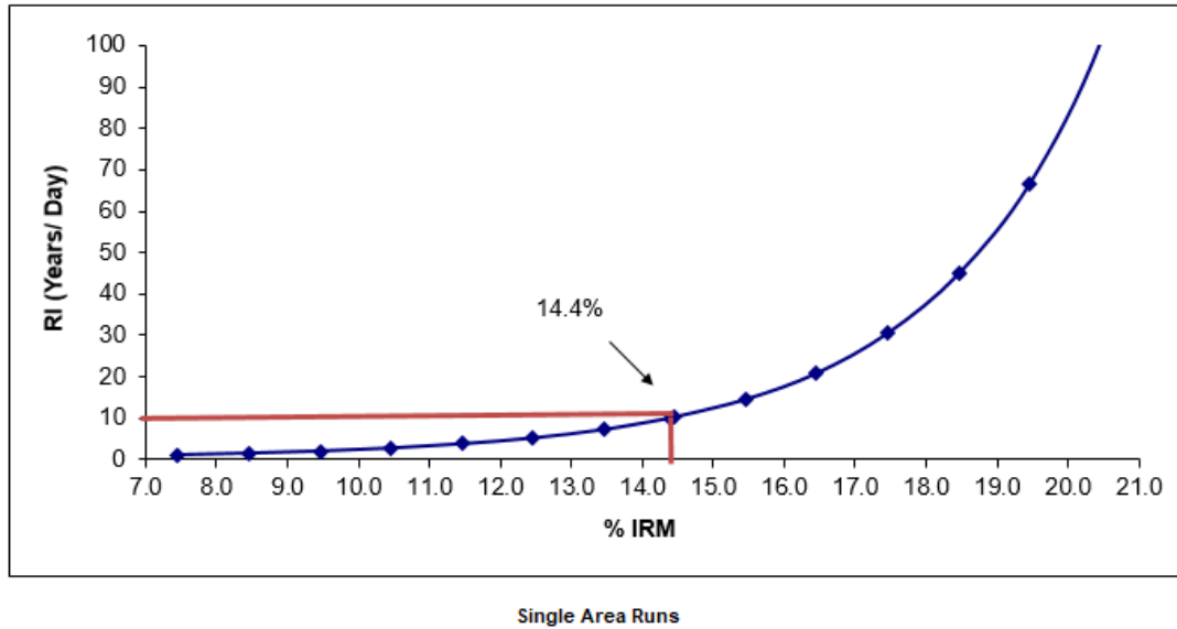
Figure II-5: Installed Reserve Margin (IRM) vs. RI (Years/Day)
