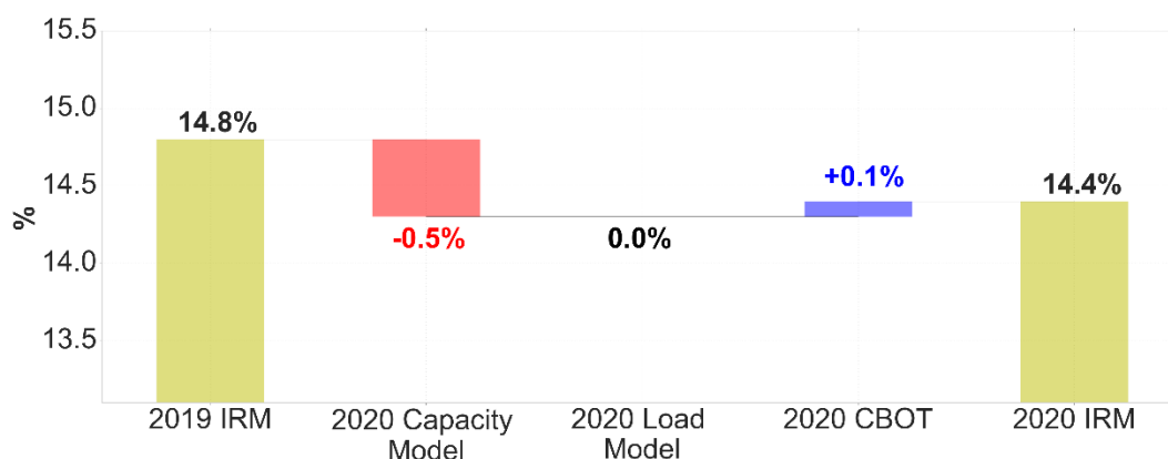
Figure I-1: 2020 Installed Reserve Margin Waterfall Chart
